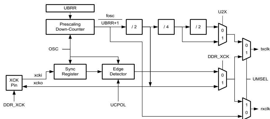
Figure 70. Clock Generation Logic, Block Diagram
