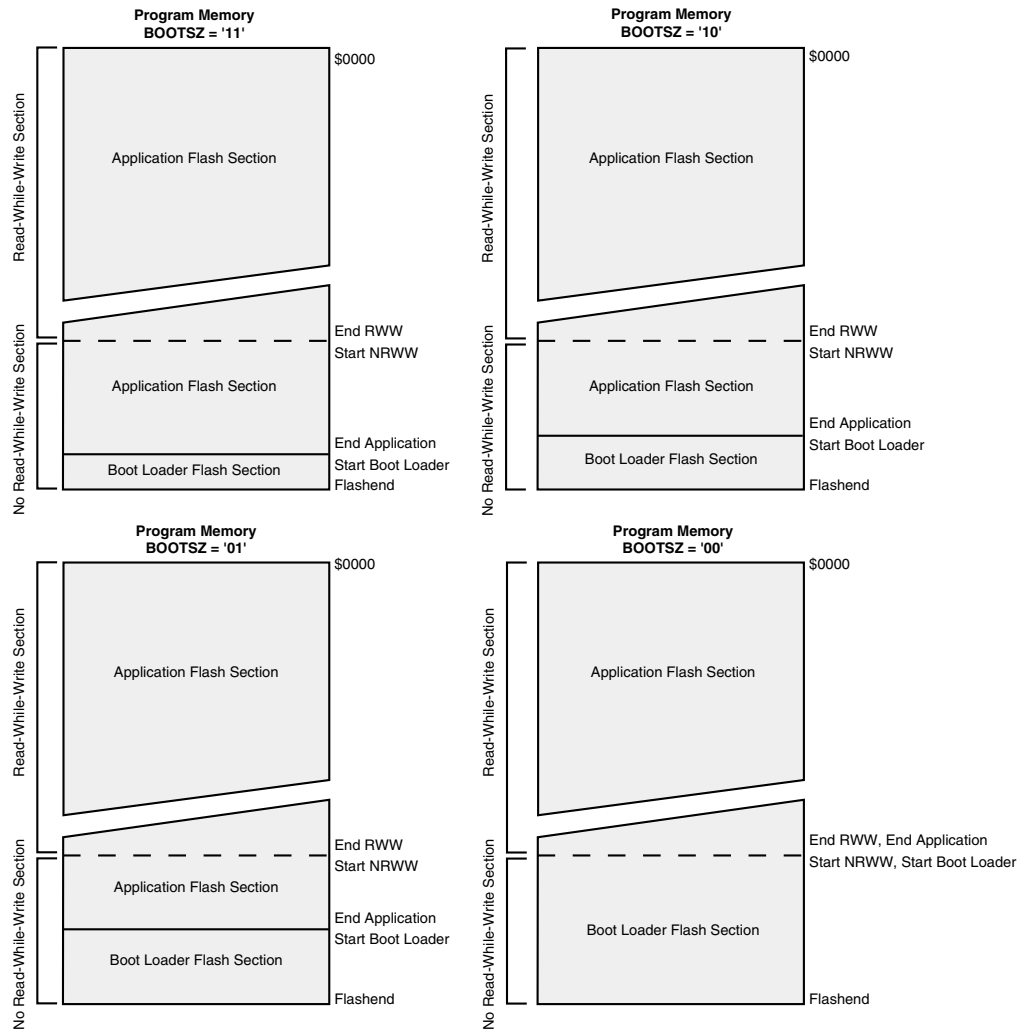
Figure 113. Memory sections (1)
