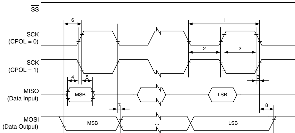
Figure 129. SPI Interface Timing Requirements (Master Mode)
