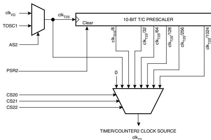
Figure 64. Prescaler for Timer/Counter2
