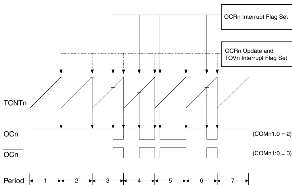
Figure 58. Fast PWM Mode, Timing Diagram
