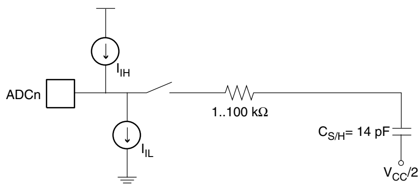
Figure 105. Analog Input Circuitry
